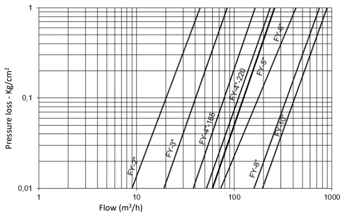
FY-M load loss, Ø2 mm pass
